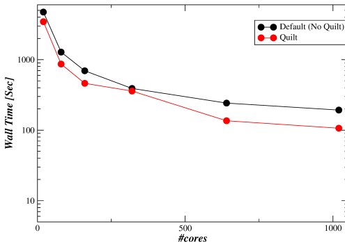
Σχήμα: WRF 3.4.1 performance : Quilting vs no Quilting
